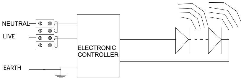
WIRING DIAGRAM FOR NON-EMERGENCY LED DRIVER
