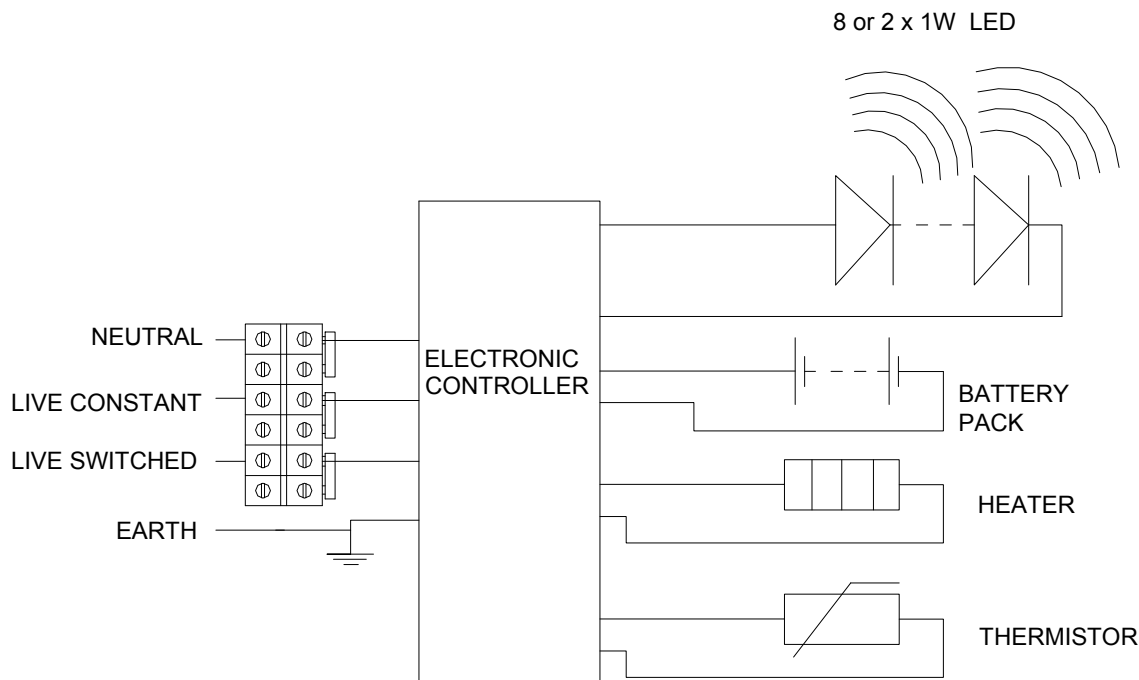
Diagram showing fully specified circuit with optional heater.
