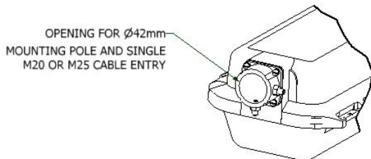
POLE MOUNT MODEL 2FT & 4FT
