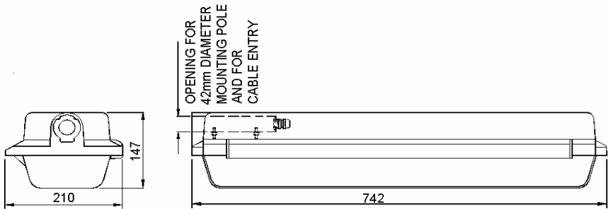
SIDE ENTRY 18/20W MODEL
